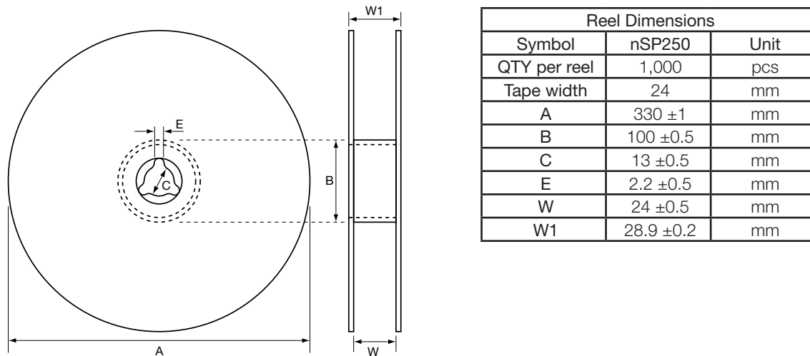
Figure 12. Reel Specifications for the nanoSplat Antenna
