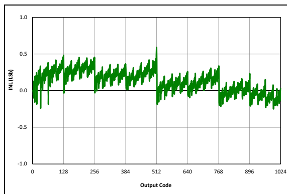
FIGURE 27-65: ADC 10-bit Mode, Single-ended INL, V_{DD} = 3.0V , T_{AD} = 1\text{ }\mu s , 25^\circ C .
