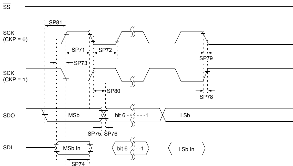
FIGURE 26-15: SPI MASTER MODE TIMING (CKE = 1, SMP = 1)
