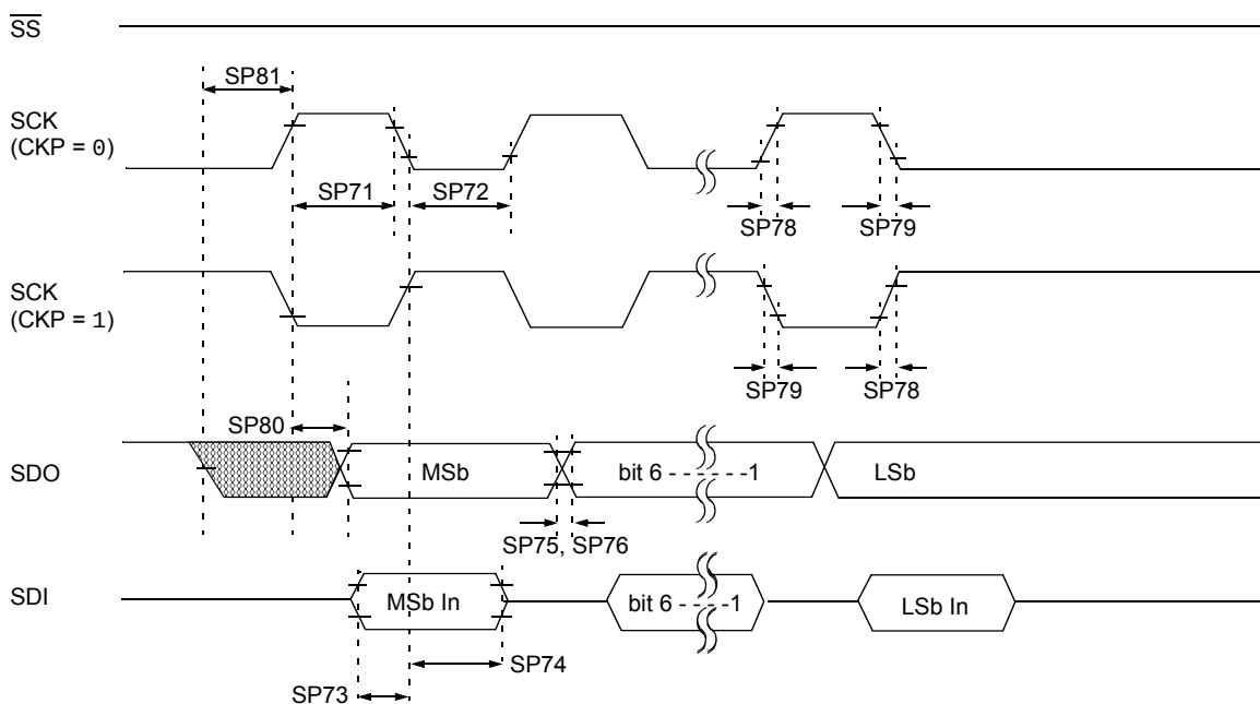
FIGURE 26-14: SPI MASTER MODE TIMING (CKE = 0, SMP = 0)
