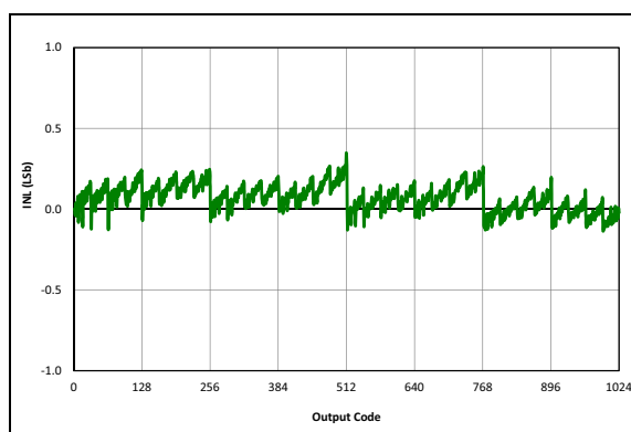
FIGURE 27-66: ADC 10-bit Mode, Single-ended INL, V_{DD} = 3.0V , T_{AD} = 4\text{ }\mu s , 25^\circ C .
