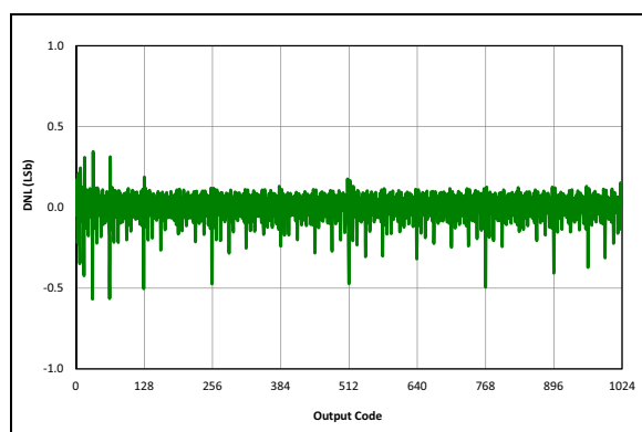
FIGURE 27-63: ADC 10-bit Mode, Single-ended DNL, V_{DD} = 3.0V , T_{AD} = 1\text{ }\mu s , 25^\circ C .
