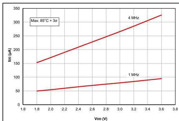
FIGURE 27-6: I_{DD} Maximum, EC Oscillator, Medium-Power Mode, PIC16F1703/7 Only.
