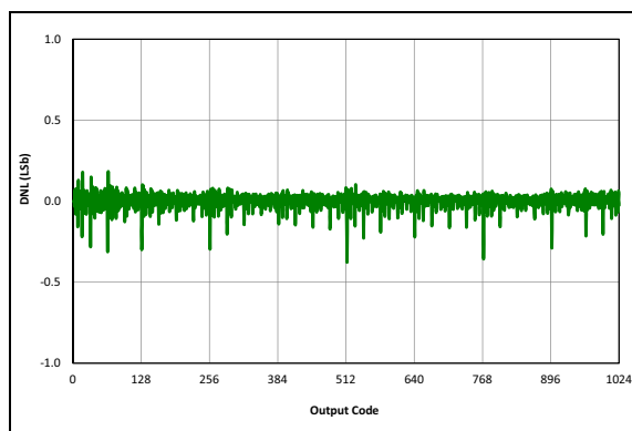
FIGURE 27-64: ADC 10-bit Mode, Single-ended DNL, V_{DD} = 3.0V , T_{AD} = 4\text{ }\mu s , 25^\circ C .
