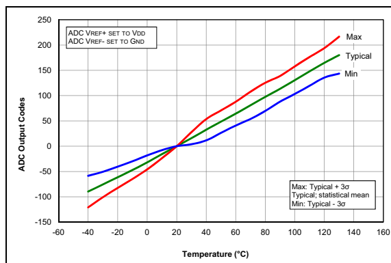
FIGURE 27-77: Temperature Indicator Slope Normalized to 20^\circ C , Low Range, V_{DD} = 1.8 , PIC16F1703/7 only.
