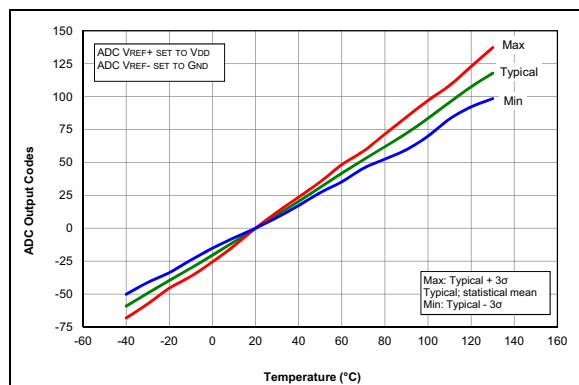
FIGURE 27-74: Temperature Indicator Slope Normalized to 20^\circ C , High Range, V_{DD} = 5.0 , PIC16F1703/7 only.
