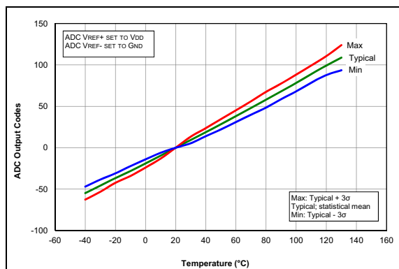
FIGURE 27-78: Temperature Indicator Slope Normalized to 20^\circ C , Low Range, V_{DD} = 3.0 , PIC16F1703/7 only.
