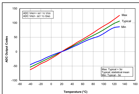
FIGURE 27-76: Temperature Indicator Slope Normalized to 20^\circ C , Low Range, V_{DD} = 3.0 , PIC16F1703/7 only.
