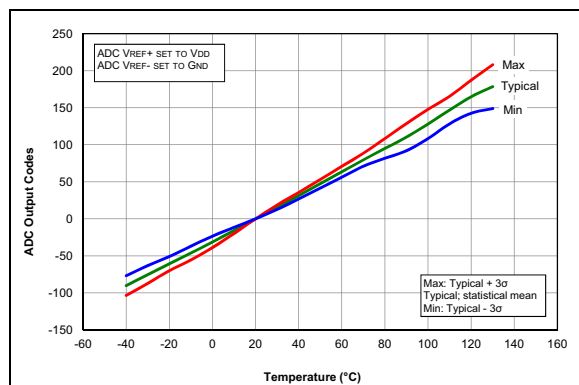
FIGURE 27-75: Temperature Indicator Slope Normalized to 20^\circ C , High Range, V_{DD} = 3.0 , PIC16F1703/7 only.
