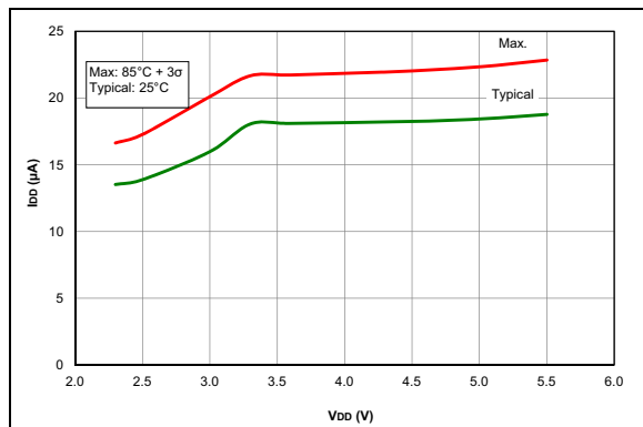
FIGURE 27-2: I_{DD} , EC Oscillator, Low-Power Mode, F_{OSC} = 32\text{ kHz} , PIC16LF1703/7 Only.
