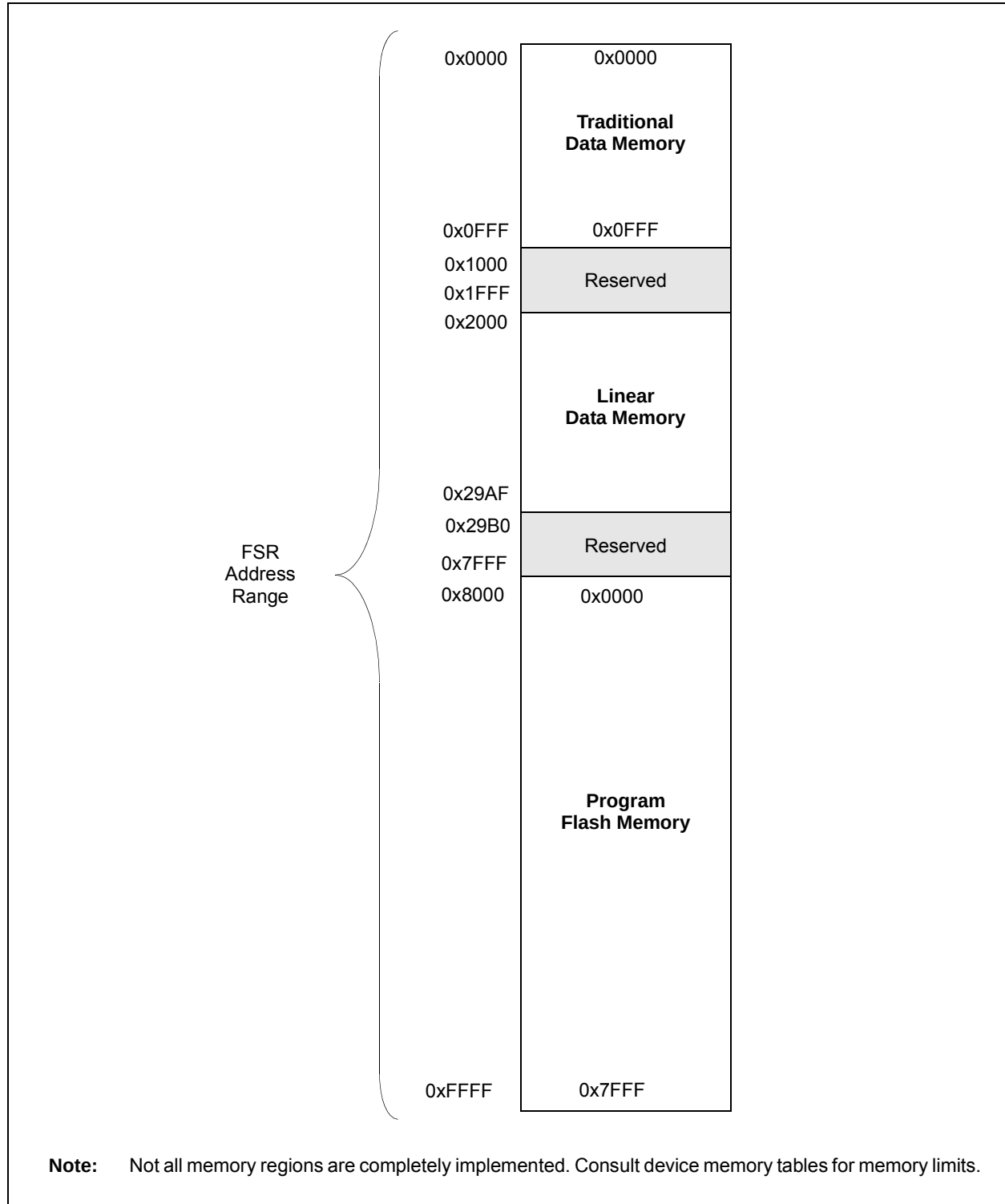
FIGURE 3-8: INDIRECT ADDRESSING
