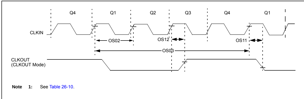
FIGURE 26-5: CLOCK TIMING
