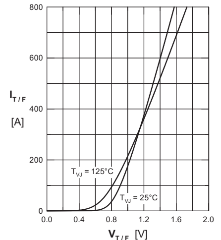
Fig. 1 Forward characteristics
