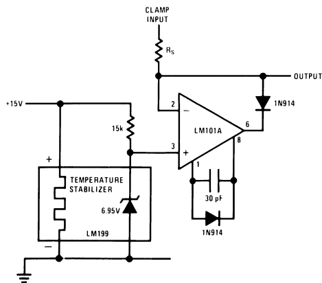
Figure 24. Precision Clamp*
