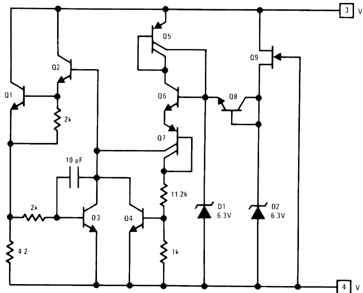
Figure 27. Temperature Stabilizer
