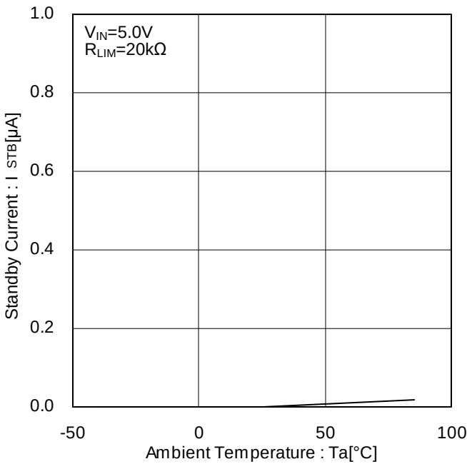
Figure 11. Standby Current vs Ambient Temperature EN Disable
