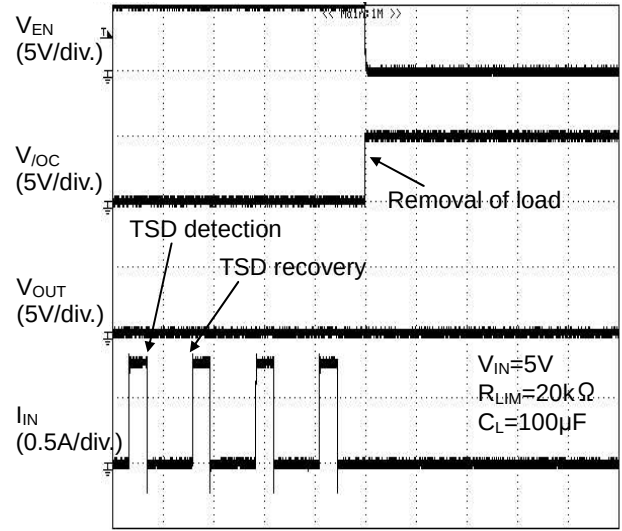
Figure 43. Over Current Response Disenable From Short Circuit (BD2242G)
