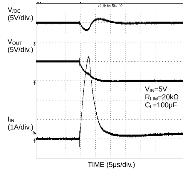
Figure 49. Over Current Response 0Ω Load Connected At Enable
