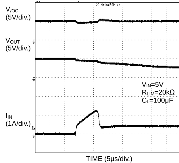
Figure 47. Over Current Response 1Ω Load Connected At Enable
