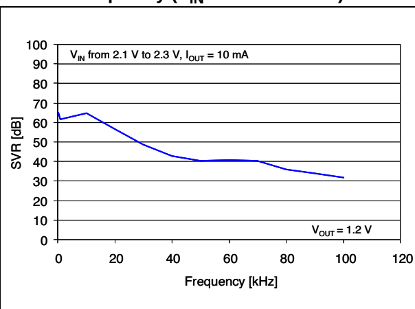
Figure 16. Supply voltage rejection vs. frequency ( V_{IN} = 2.1\text{ V to }2.3\text{ V} )
