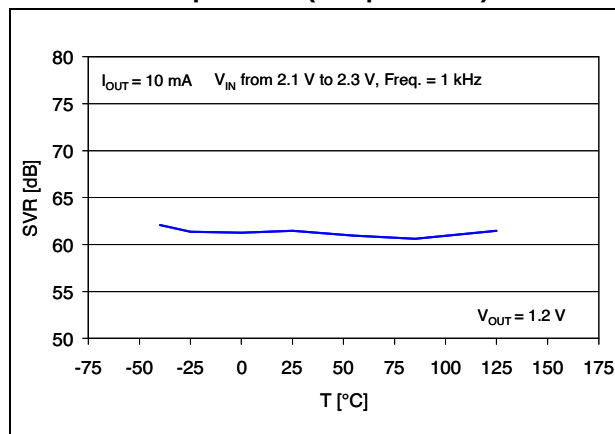
Figure 13. Supply voltage rejection vs. temperature (Freq. = 1 kHz)
