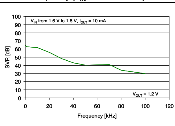
Figure 14. Supply voltage rejection vs. frequency ( V_{IN} = 1.6\text{ V to }1.8\text{ V} )
