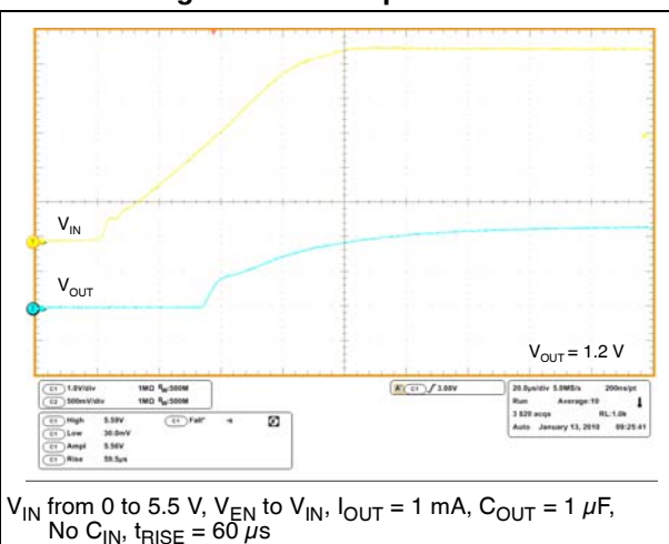
Figure 20. Startup transient
