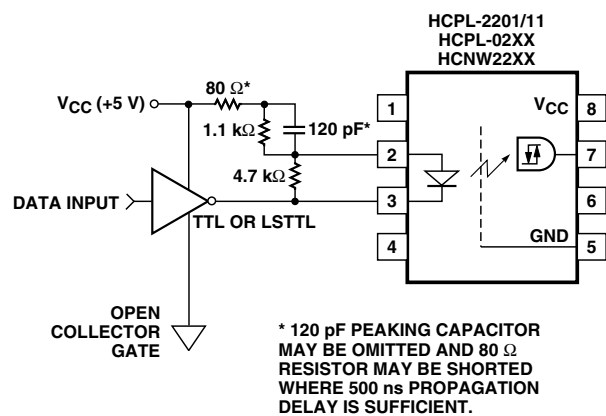
Figure 16. Series LED drive with open collector gate ( 4.7\ \text{k} resistor shunts I_{OH} from the LED).
