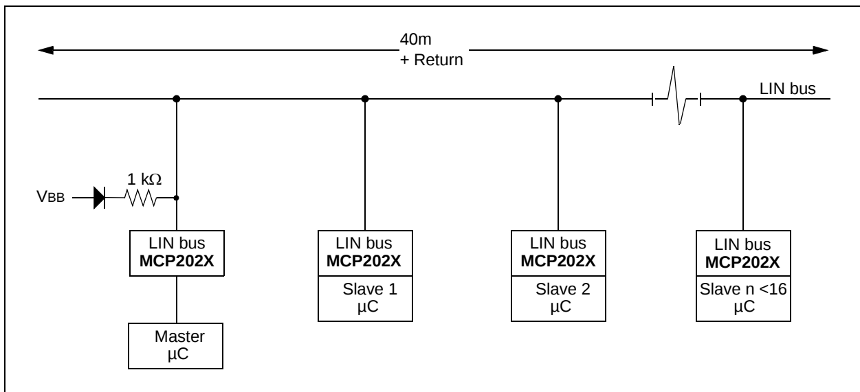
FIGURE 1-7: Typical MCP2022/MCP2022P Application.
