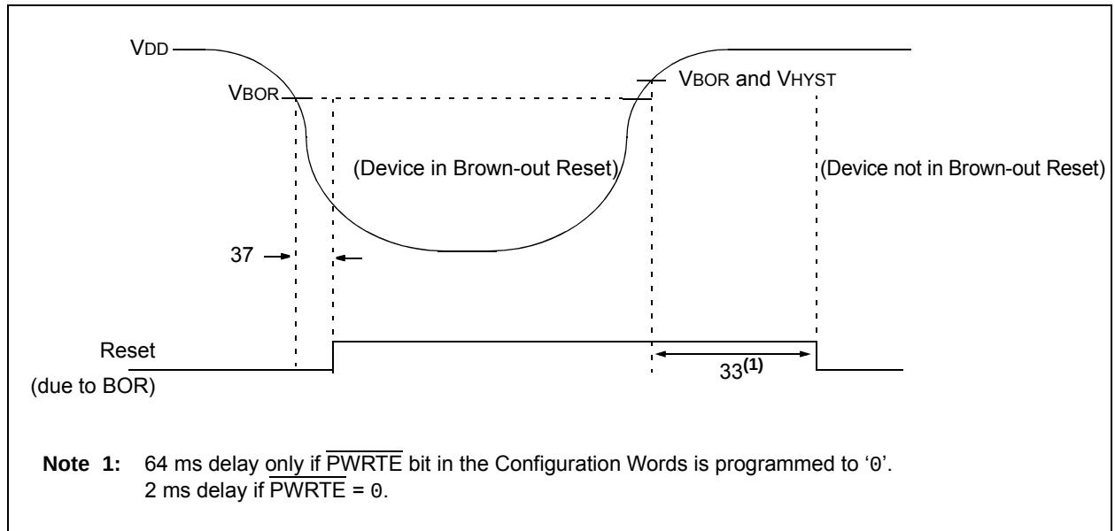
FIGURE 25-7: BROWN-OUT RESET TIMING AND CHARACTERISTICS
