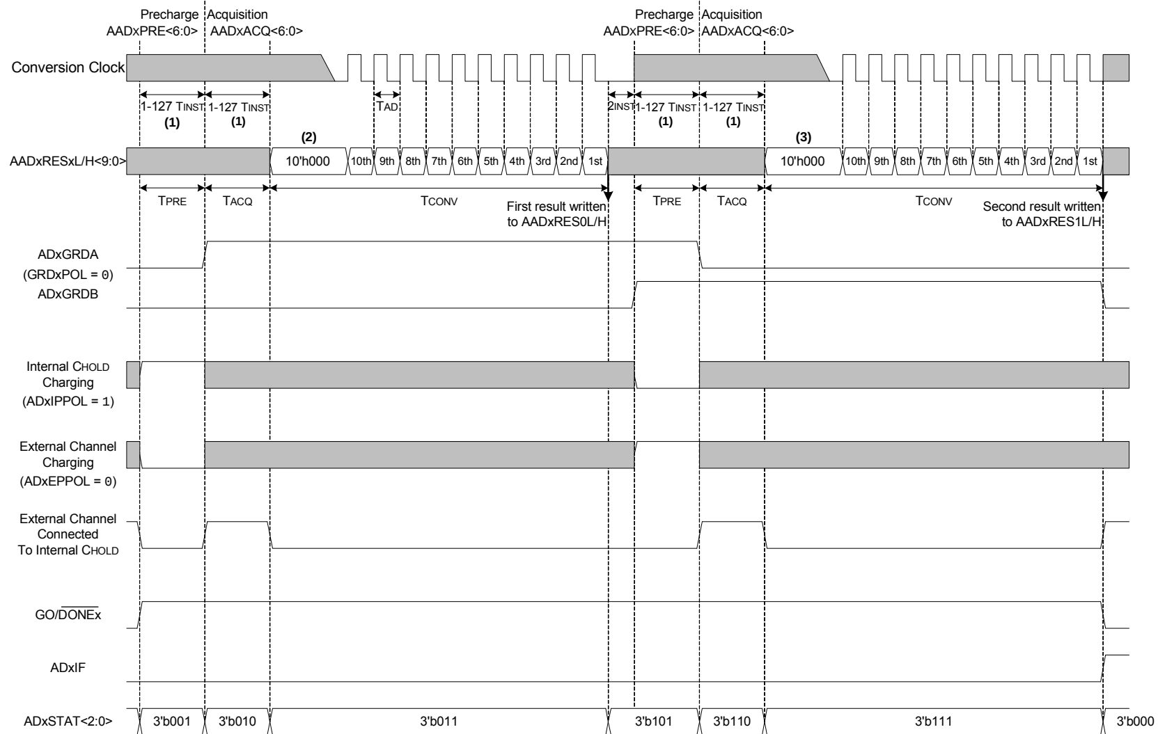
FIGURE 16-7: DOUBLE SAMPLE CONVERSION SEQUENCE (ADDSSEN = 1 AND ADIPEN = 1)
