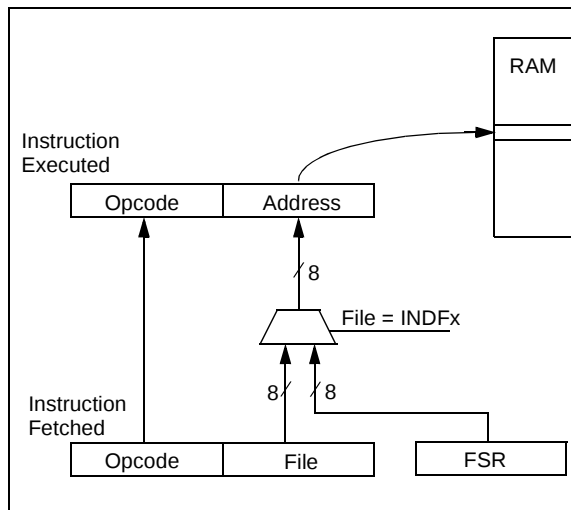
FIGURE 7-6: INDIRECT ADDRESSING
