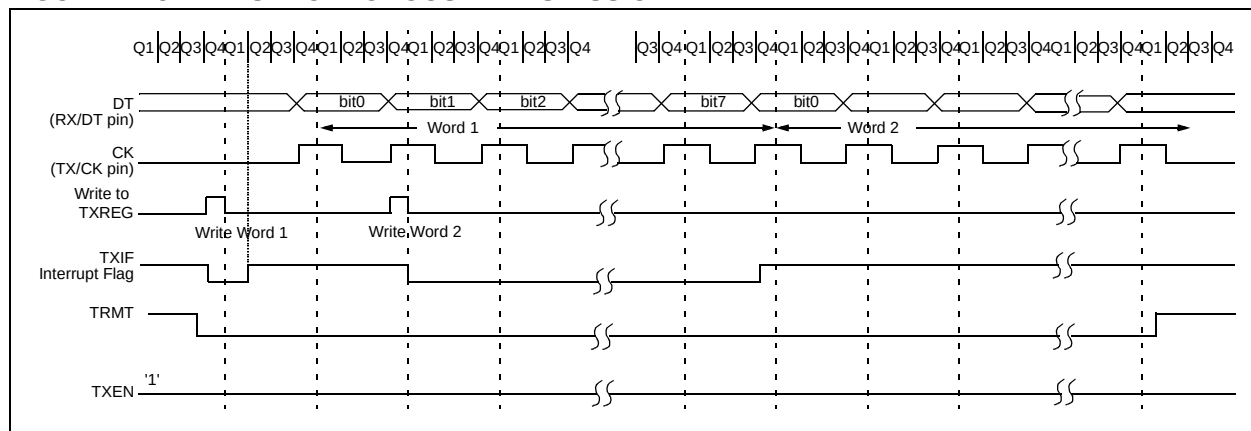
FIGURE 14-8: SYNCHRONOUS TRANSMISSION
