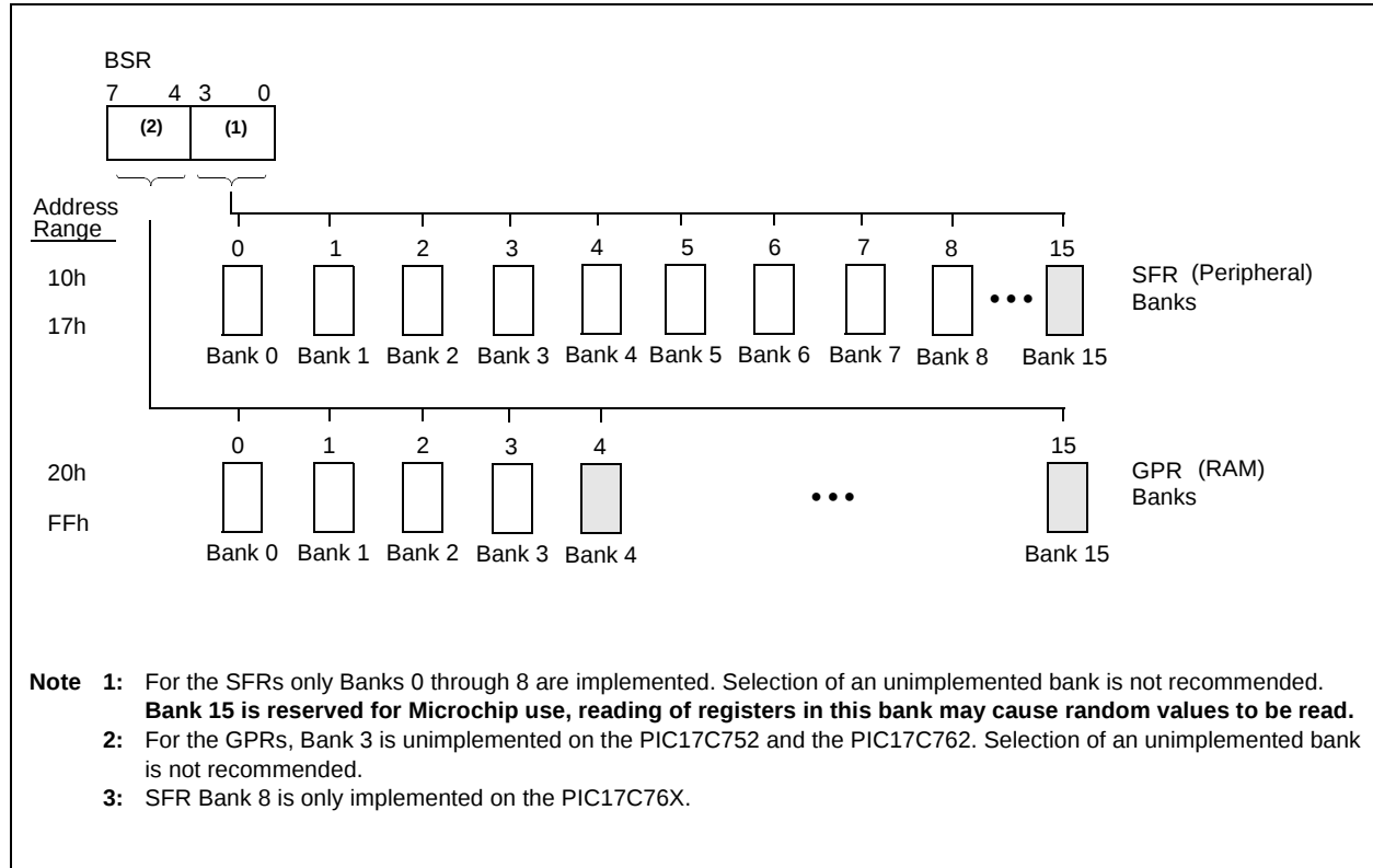
FIGURE 7-9: BSR OPERATION
