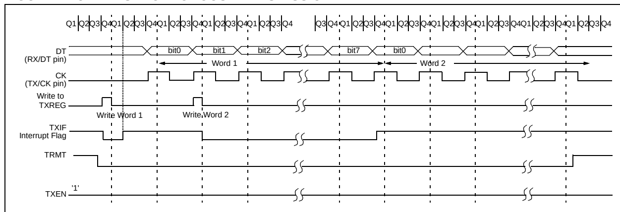
FIGURE 14-8: SYNCHRONOUS TRANSMISSION
