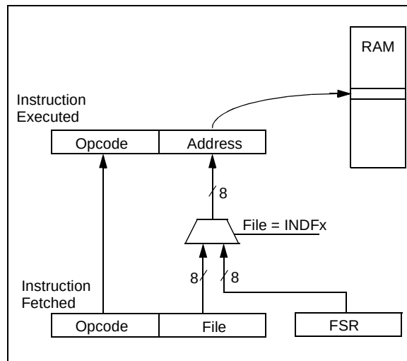
FIGURE 7-6: INDIRECT ADDRESSING
