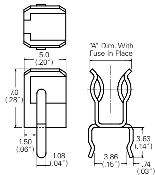
111 501 / 111 506 Device Dimensions
