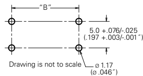
Recommended Mounting Dimensions
