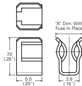
111 505 Device Dimensions
