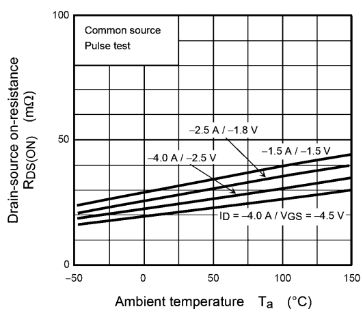
Fig. 7.5 R_{DS(ON)} - T_a
