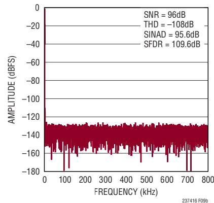
Figure 9b. 32k Point FFT f_{\text{SAMPL}} = 1.6\text{Msps} , f_{\text{IN}} = 1\text{kHz} for Circuit Shown in Figure 9a
