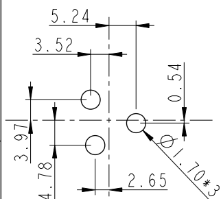
3Pin Male Connector Male Pin PCB Layout
