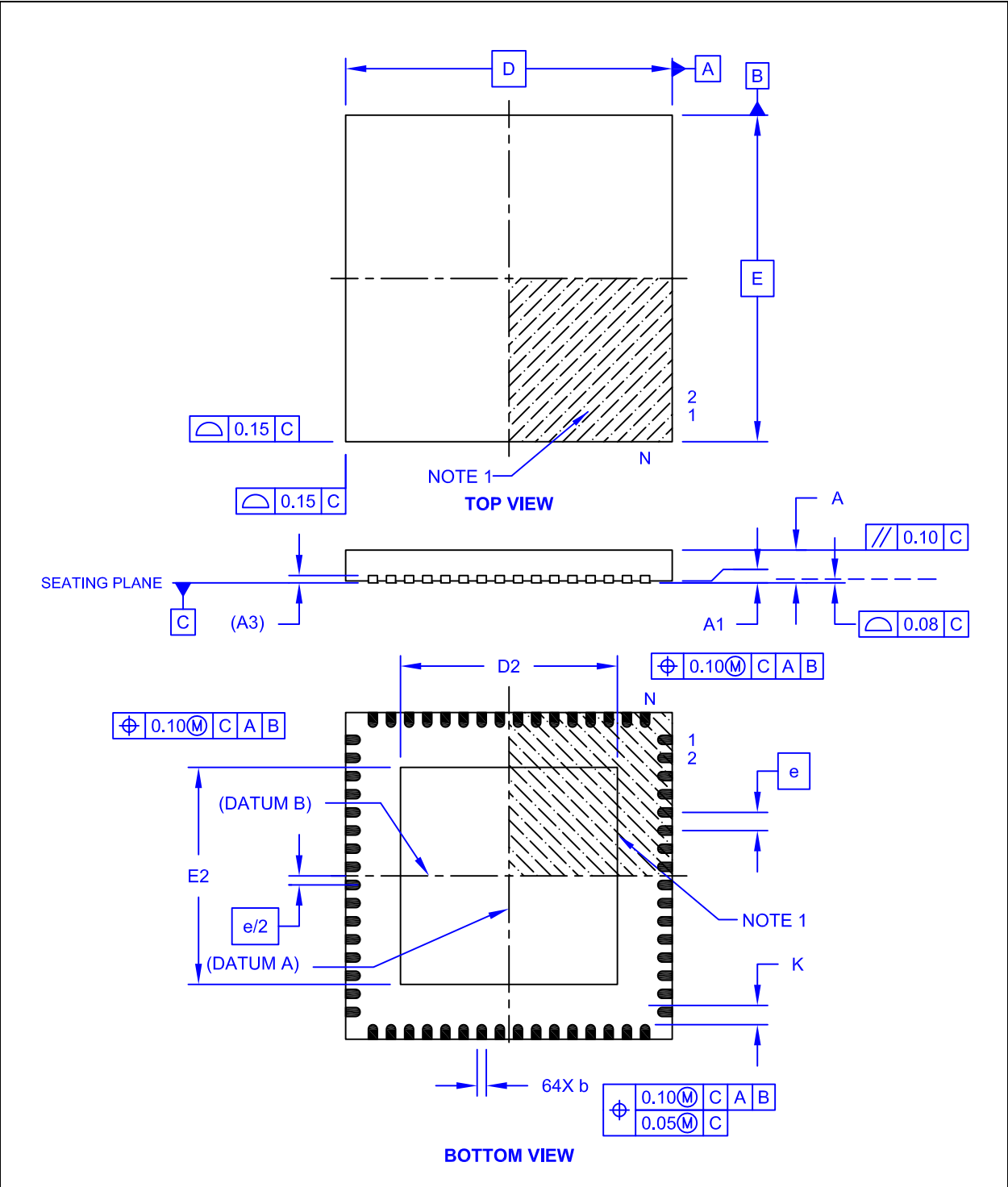
FIGURE 20-1: 64-QFN PACKAGE
