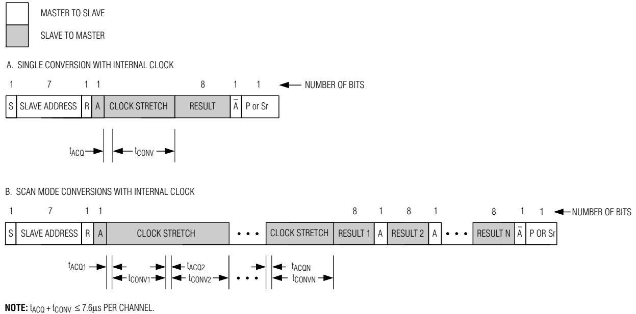
Figure 10. Internal Clock Mode Read Cycles
