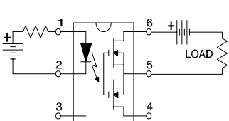
"B" Connection
