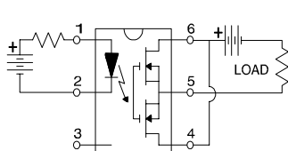
"C" Connection
