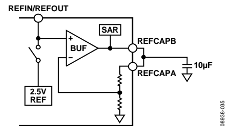
Figure 37. Reference Circuitry
