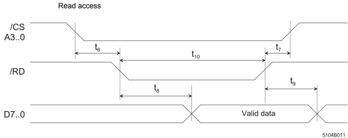
Figure 3-3 Timing for read access
