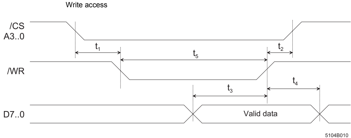
Figure 3-2 Timing for write access
