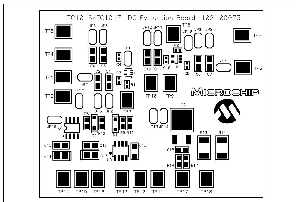
FIGURE 2-1: TC1016/TC1017 LDO Evaluation Board Assembly Layout.
