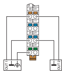
Connection diagram
