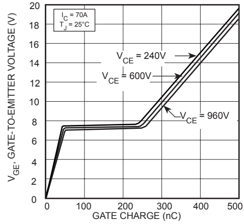
FIGURE 11, Gate charge
