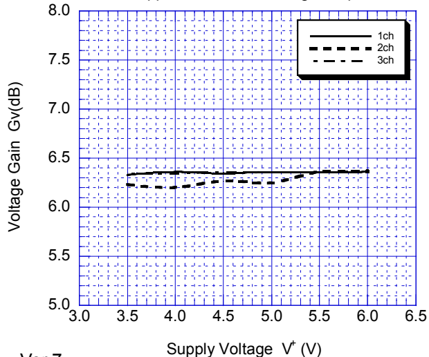
Voltage Gain vs. Supply Voltage
