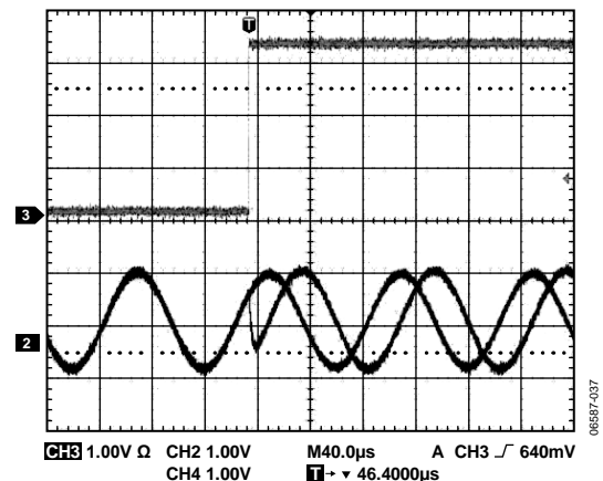
Figure 38. Phase Switching Response at 90° (Top: CSB)
