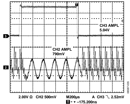
Figure 36. LO Reset Response (see Figure 45)
