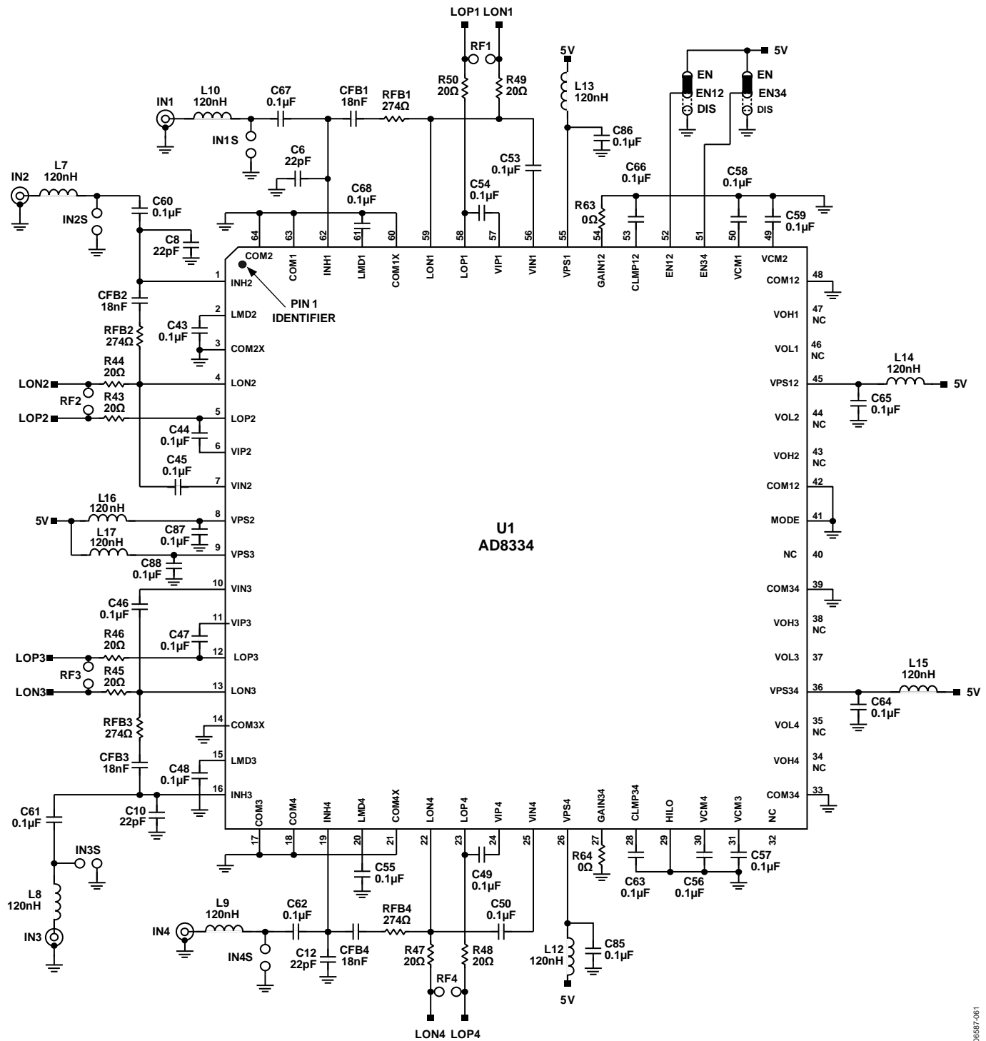
Figure 63. Schematic—LNA Section
