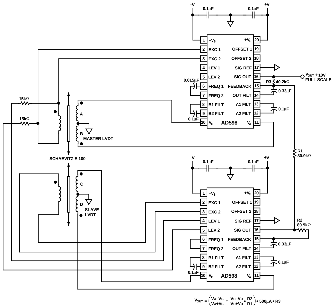
Figure 26. Precision Differential Gaging
