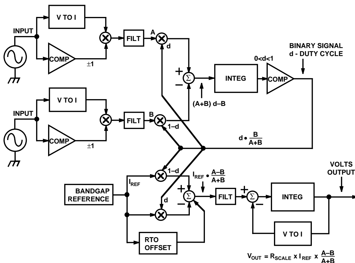
Figure 6. Block Diagram of Decoder
