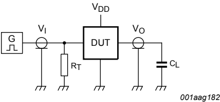
Test data is given in Table 10. Definitions for test circuit: C L = load capacitance including jig and probe capacitance. R T = termination resistance should be equal to the output impedance Z o of the pulse generator.
