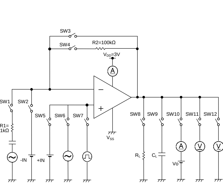
Figure 68. Test Circuit 2
