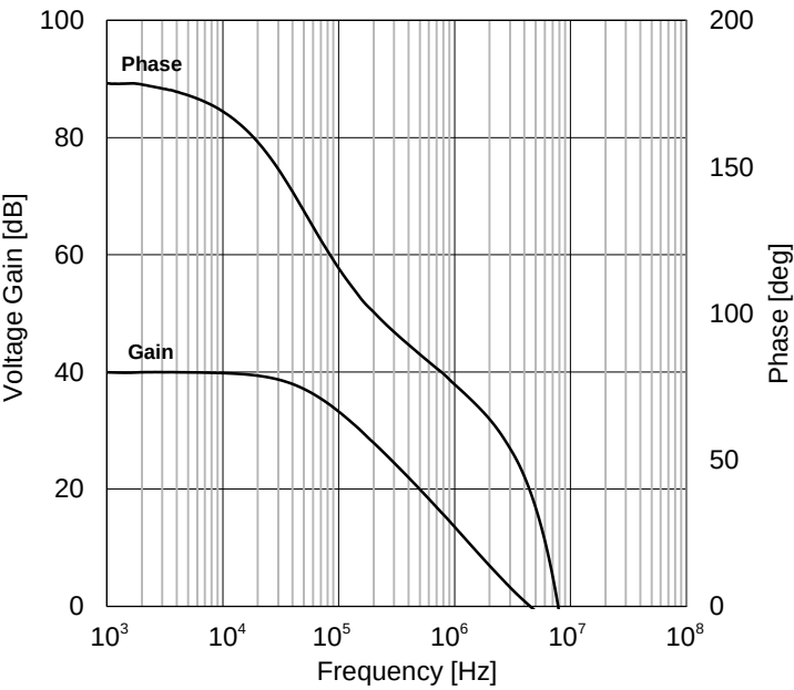
Figure 66. Voltage Gain · Phase vs Frequency
