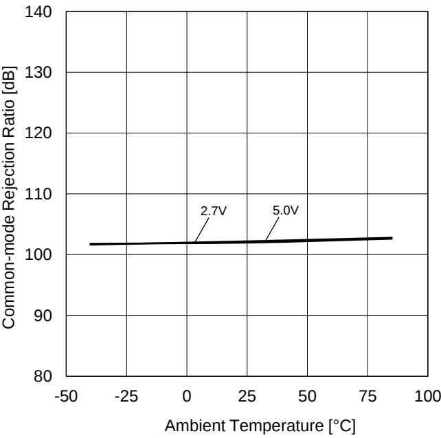
Figure 40. Common-mode Rejection Ratio vs Ambient Temperature
