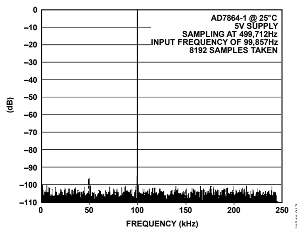
Figure 17. FFT Plot
