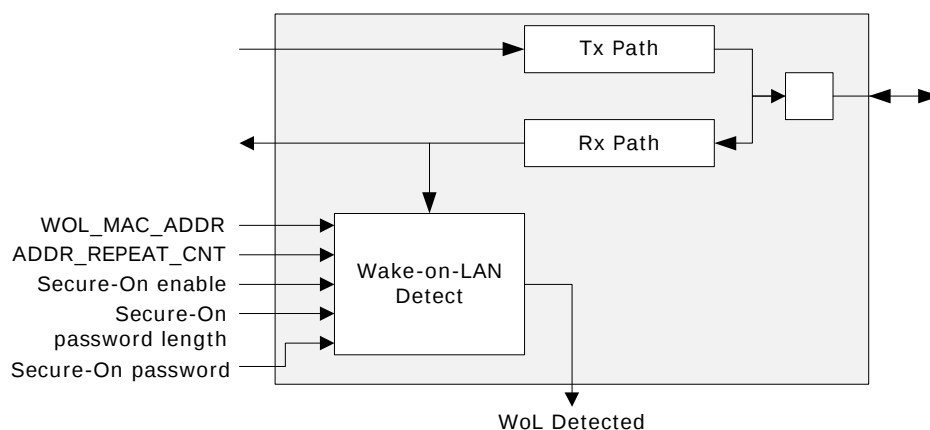
Figure 17 • Wake-on-LAN Functionality
