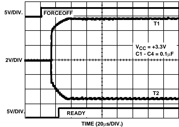
FIGURE 10. TRANSMITTER OUTPUTS WHEN EXITING POWERDOWN
