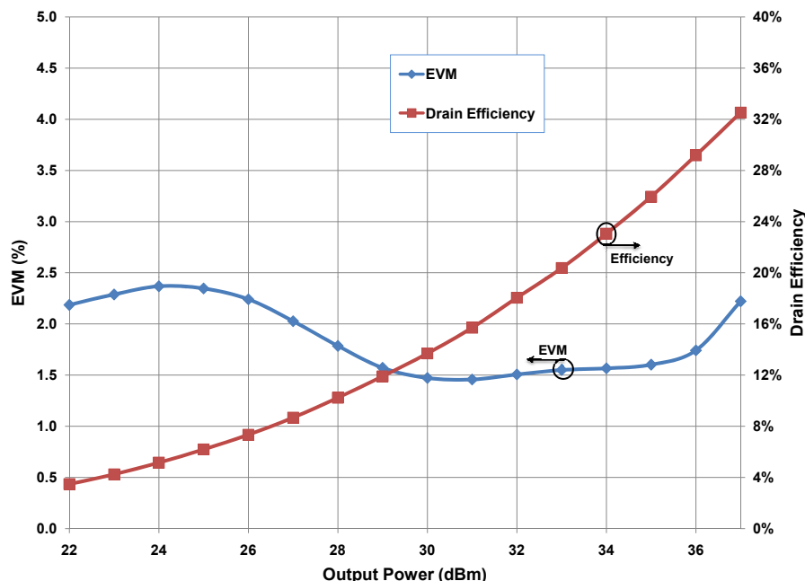
Drain Efficiency and EVM vs Output Power measured in CGH27030F-AMP V_{DD} = 28\text{ V} , I_{DQ} = 150\text{ mA} , 802.16-2004 OFDM, PAR = 9.8 dB
