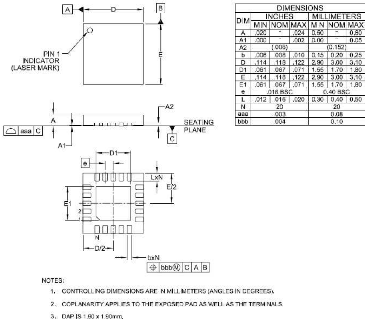
Figure 14: Outline Drawing
