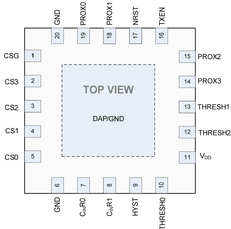
Figure 1: Pin Diagram
