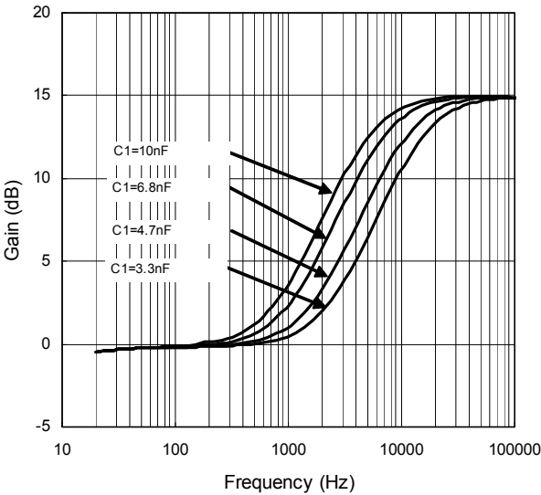
Gain vs Frequency (TONE TREBLE )
