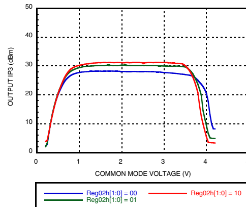
Figure 22. Output IP3 vs Output Common Mode Voltage, 70 MHz Input [9]
