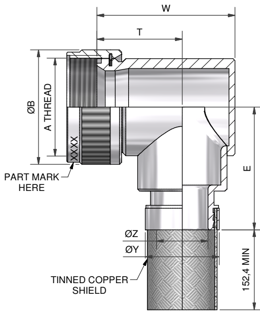
90° BACKSHELL - TYPE 1
