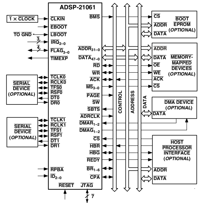
Figure 2. ADSP-21061/ADSP-21061L System Sample Configuration
