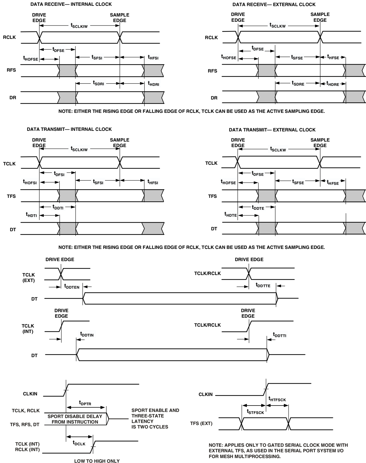
Figure 24. Serial Ports
