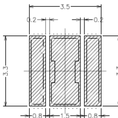
Soldering patterns
