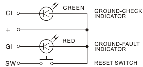
INTERNAL SCHEMATIC
